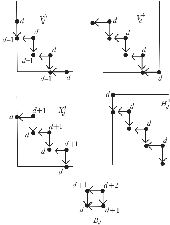
Figure 3. Examples of possible summands of an E_2 -collapsed chain complex.
