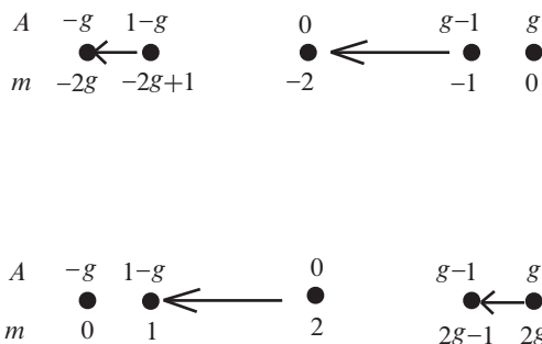
Figure 5. Different possibilities for \widehat{\text{CFK}}(L_2; \mathbb{Q}) : here, we denote the Alexander grading of the generators by A and the Maslov grading by m .
