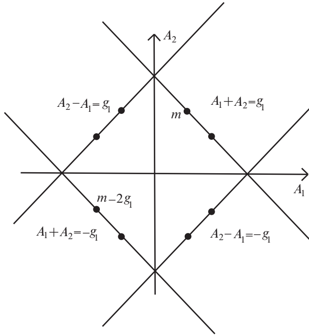
Figure 4. A rank eight bigraded vector space not arising as the link Floer homology of a link.
