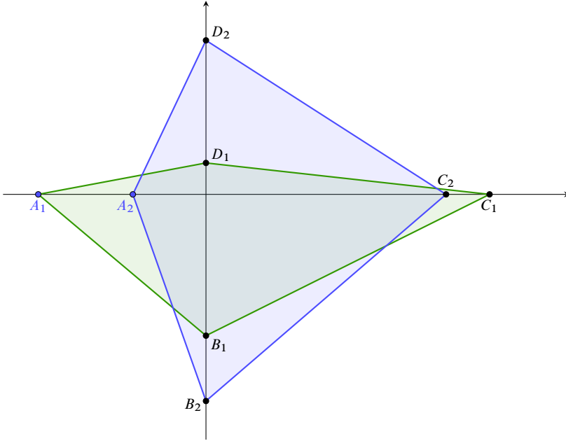
Figure 4. Two possible shapes of an orthodiagonal four-bar linkage ABCD , the coordinate axes are fixed “tracks” on which the points can move
