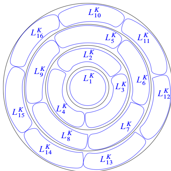
Figure 3. The sequence \underline{L}^k .
