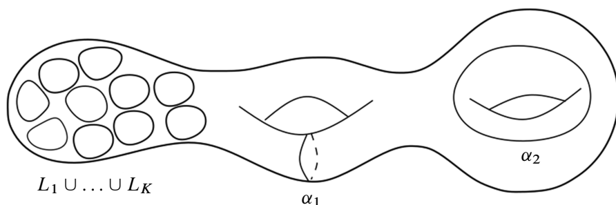
Figure 1. An admissible link.
