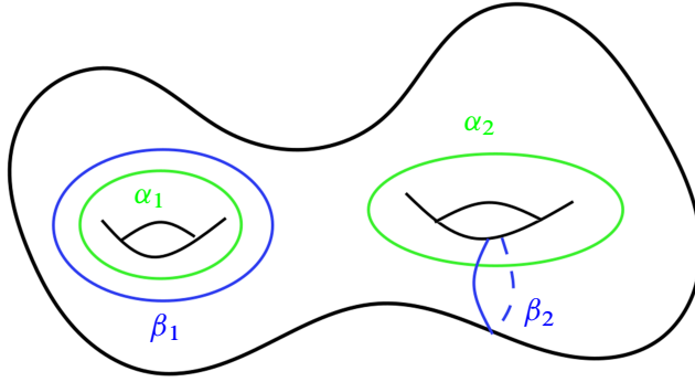
Figure 2. Two links \underline{\alpha} and \underline{\beta} inducing independent invariants \mu_{\underline{\alpha}} and \mu_{\underline{\beta}} .
