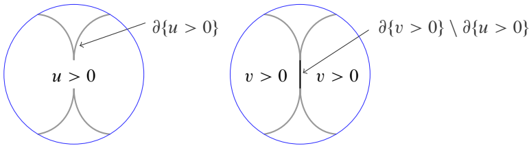
Figure 1. An illustration of uncoupled free boundary points shaped in a singular fashion. All regular free boundary points are in the coupled free boundary.
