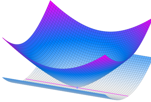
Figure 2. An illustration of a nonempty uncoupled free boundary \partial\{v > 0\} \setminus \partial\{u > 0\} (see Example 4). The red line above is \partial\{v > 0\} and the blue point is \partial\{u > 0\} . By Theorem 6.3, all points on \partial\{v > 0\} \setminus \partial\{u > 0\} are singular. In this example, there are no regular points.
