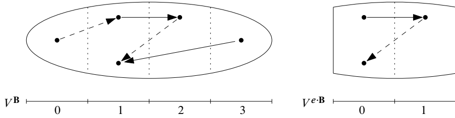
Fig. 2. An example of forming e \cdot \mathbf{B} from e and \mathbf{B} . Left: \mathcal{L}_4 -structure \mathbf{B} , right: \mathcal{L}_2 -structure e \cdot \mathbf{B} , where e: 4 \rightarrow 2 with \text{dom}(e) = \{1, 2\} , e(1) = 0 , e(2) = 1 .
