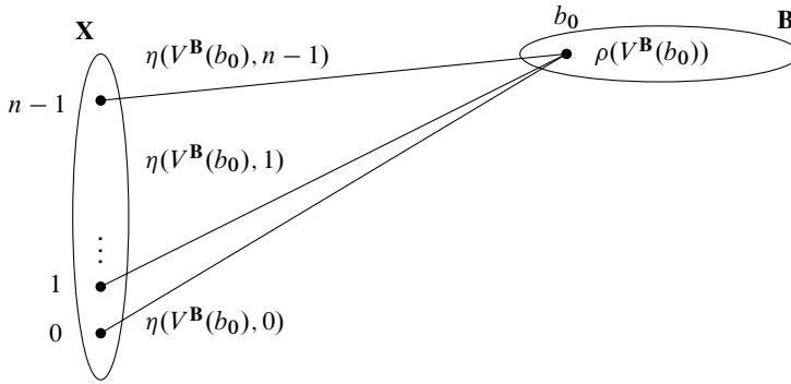
Fig. 1. A gluing (\mathbf{X}, \rho, \eta) with X = \{0, \dots, n-1\} .
