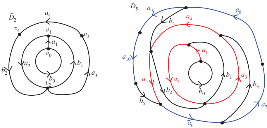
Figure 4. Discs \tilde{D}_2 and \tilde{D}_5 . In \tilde{D}_5 we identify b_5 with b_0 and the blue path with the red one to get \tilde{C}_5 .
