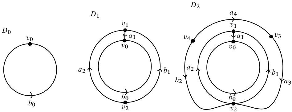
Figure 2. Discs D_0 , D_1 and D_2 with their labelings.
