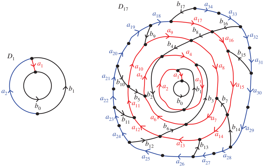
Figure 3. In D_{17} we identify b_{17} with b_0 and the blue path with the red one to get C_{17} . Similarly for D_1 .
