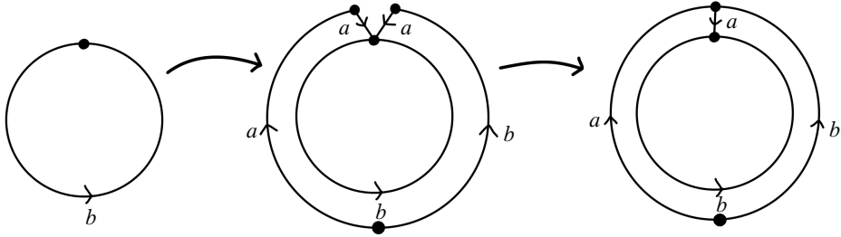
Figure 1. Coupling a 2-cell of type 2 to a 2-cell of type 1.
