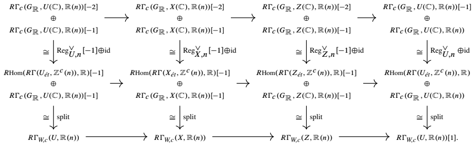
Figure 3. Diagram induced by a closed-open decomposition Z \not\leftrightarrow X \leftrightarrow U .
