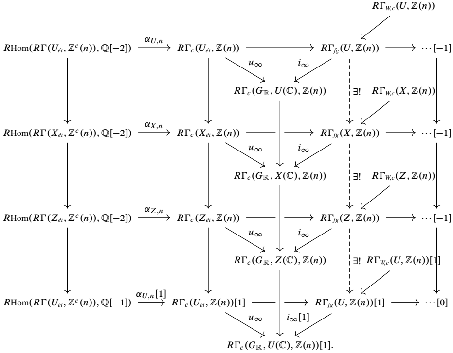
Figure 1. Diagram induced by a closed-open decomposition Z \not\leftrightarrow X \leftrightarrow U .
