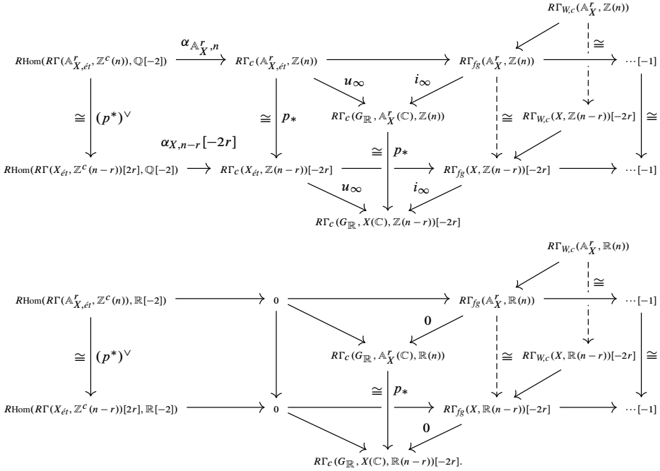
Figure 4. Isomorphism R\Gamma_{W_C}(\mathbb{A}_X^r, \mathbb{Z}(n)) \cong R\Gamma_{W_C}(X, \mathbb{Z}(n-r))[-2r] and its splitting after tensoring with \mathbb{R} .
