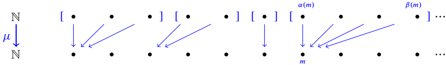
Figure 1. Schematic of the map \mu .
