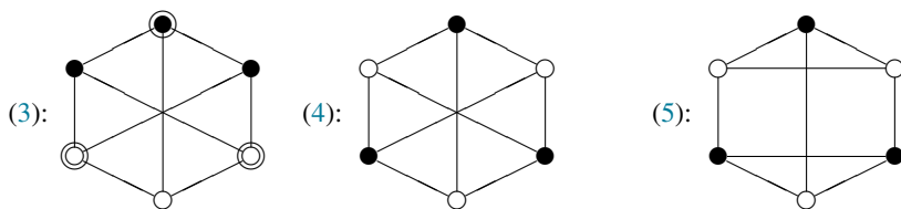
FIGURE 4. The intersection of M'_3 with the pre-images of the diagonals.
