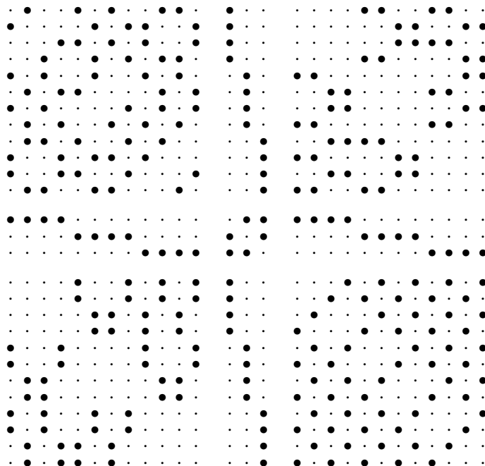
FIGURE 3. The 27 invariant divisors.
