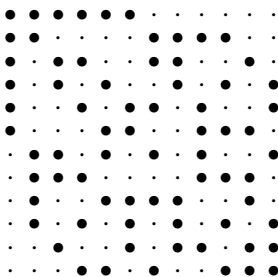
FIGURE 1. The graph \Gamma_2 .
