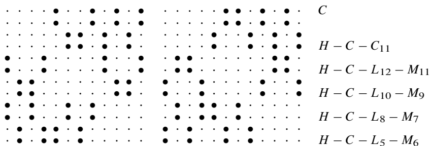
FIGURE 2. The twelve new conics.
