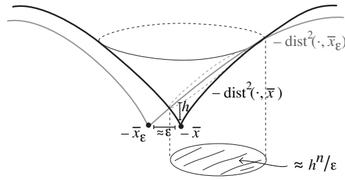
Fig. 1. On the sphere, the squared distance function from a point \bar{x} looks like a cone near -\bar{x} . So, if \text{dist}(\bar{x}, \bar{x}_\varepsilon) = \text{dist}(-\bar{x}, -\bar{x}_\varepsilon) \approx \varepsilon , the section obtained by cutting its graph with -\text{dist}^2(\cdot, \bar{x}_\varepsilon) at height h has measure \approx h^n/\varepsilon .
