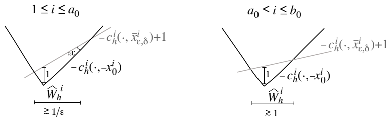
Fig. 3. If 1 \leq i \leq a_0 then -x_0^i = \bar{x}_0^i and \text{dist}_i(-x_0^i, \bar{x}_{\varepsilon,\delta}^i) \approx \varepsilon , so the size of the section is of order 1/\varepsilon (see also Figure 1). On the other hand, if a_0 < i \leq b_0 then -x_0^i \neq \bar{x}_0^i , which implies that \text{dist}_i(-x_0^i, \bar{x}_{\varepsilon,\delta}^i) is uniformly bounded away from 0, and the size of the section is of order 1.
