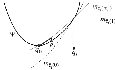
Fig. 4. The supporting function m_{\bar{z}_i(0)} = m_{\bar{z}_i} touches \varphi at q_i from below. By interpolating between m_{\bar{z}_i} = m_{\bar{z}_i(0)} and m_{\bar{x}_{\varepsilon,\delta}} = m_{\bar{z}_i(1)} along the \tilde{c} -segment with respect to q_i , we can find \tau_i \in [0, 1) such that m_{\bar{z}_i(\tau_i)}(q_0) = \varphi(q_0) . Then the covector \hat{p}_i used to construct \tilde{C} is defined as \hat{p}_i := (0, -D_{q_0} \tilde{c}''(q_0'', \bar{z}_i''(\tau_i))) \in \partial m_{\bar{z}_i(\tau_i)}(q_0) .
