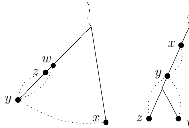
Fig. 5. The two configurations of \delta -forks with large contraction of the prongs.
