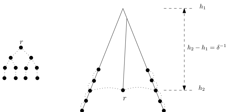
Fig. 2. The metric space on the right is the H -tree (B_\infty, d_\varepsilon) , where \varepsilon_n = \delta for all n . The picture describes an embedding of the tree on the left ( B_3 minus four leaves) into (B_\infty, d_\varepsilon) with distortion at most 6, yet all ancestor/descendant distances are distorted by at most 1 + O(\delta) .
