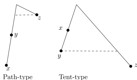
Fig. 3. A schematic description of path-type and tent-type configurations.
