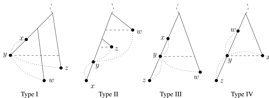
Fig. 4. The four “problematic” types of \delta -forks.
