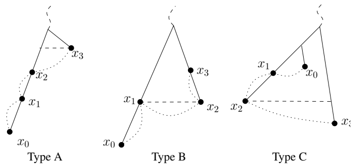
Fig. 6. The three possible types of approximate 3-paths.
