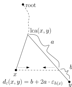
Fig. 1. The metric d_\varepsilon defined on B_\infty . The arrows indicate horizontal contraction by \varepsilon_{h(x)} .
