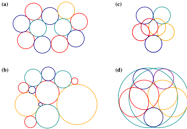
Fig. 1. An illustration of the four coloring problems of tangency graphs of constellations: (a) a penny graph, (b) a coin graph, (c) an overlapping penny graph, and (d) a general constellation as in the circle problem.
