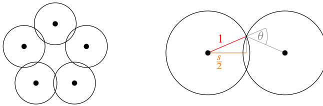
Fig. 2. In a regular n -gon of sidelength s , the circles intersect at an angle of \theta = \pi - 2 \arcsin(\frac{s}{2}) .
