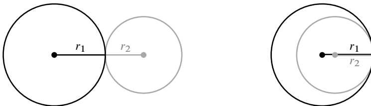
Fig. 6. External and internal tangency of circles.
