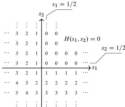
Fig. 6.1. The H -function of the Hopf link
