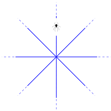
Figure 2. The infinite star-like graph K_{1,k} with k = 8 edges. Walsh's sticky process on K_{1,k} is a Feller process whose behavior at the graph's center is characterized by the boundary condition visible above; outside of the center, on each of the edges, the process behaves like a standard one-dimensional Brownian motion.
