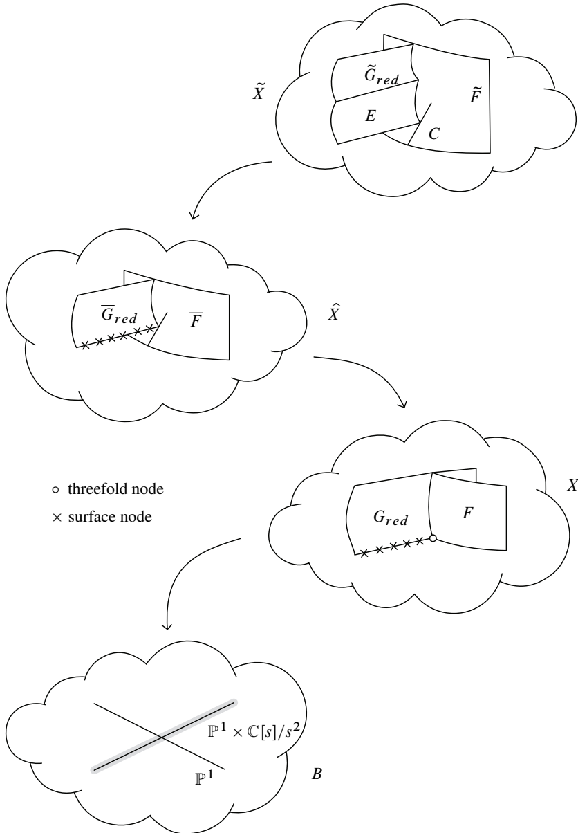
Figure 1. Constructing the resolution. Here, \overline{F} , \overline{G}_{\text{red}} denote the strict transforms in \hat{X} and \tilde{F} , \tilde{G}_{\text{red}} denote the strict transforms in \tilde{X} .
