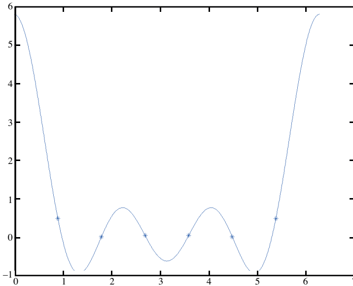
Figure 2. The graph of the symbol function 1 + 2(1 - h) \cos \varphi + 2(1 - 2h) \cos(2\varphi) + 2(1 - 3h) \cos(3\varphi) ( h = 1/10 , n = 4 ). The asterisks are the values of the function at \varphi_\ell = 2\pi\ell/7 .
