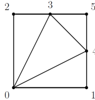
FIGURE 2. A coherent triangulation of \rho(A) from Example 6.11.
