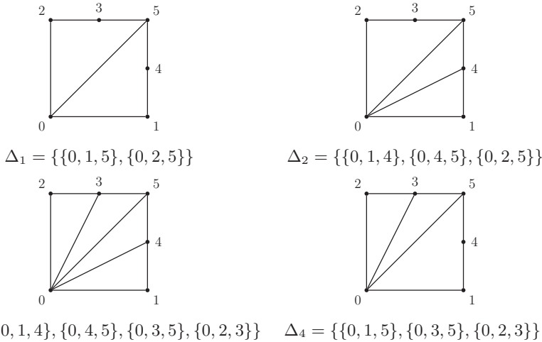
FIGURE 1. The coherent triangulations of \rho(A) corresponding to perturbations of the vector (0, 1 \dots, 1) for Example 6.11.
