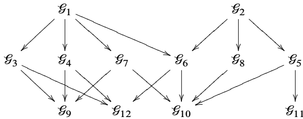
Figure 1. Lattice of finite subgroups in GL_2(\mathbb{Z}) .
