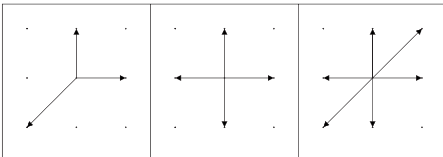
Figure 1. Lattice of finite subgroups in GL_2(\mathbb{Z}) .
