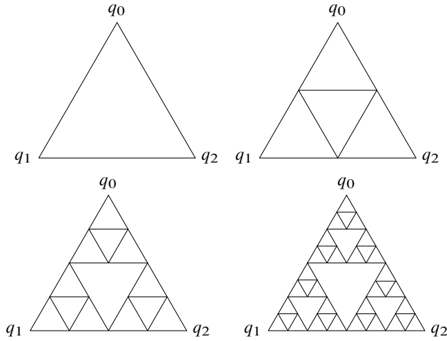
Figure 1.1. Left to right: \Gamma_0, \Gamma_1, \Gamma_2, \Gamma_3 of SG.
