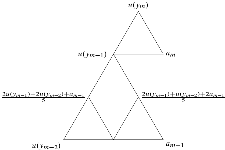
Figure 2.2. Harmonic extension.
