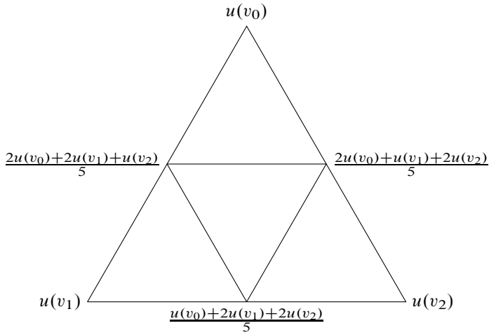
Figure 2.1. Harmonic Extension Algorithm.
