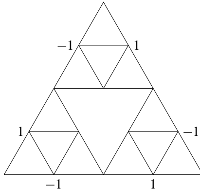
Figure 5.1. Odd eigenfunction on \Gamma_2 .
