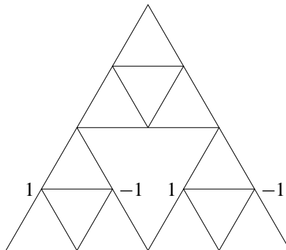
Figure 5.2. Another odd eigenfunction on \Gamma_2 .
