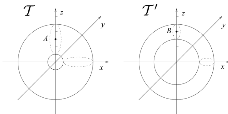
Fig. 1. In this case an optimal homeomorphism (i.e. one minimizing \Theta ) exists and d = 2 ; d equals the distance between a critical value of \varphi and a critical value of \varphi' .
