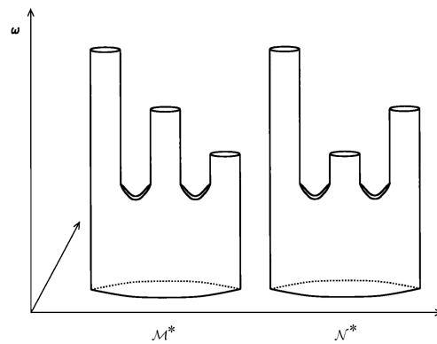
Fig. 10. The metrics \mu_{\mathcal{M}^*} and \mu_{\mathcal{N}^*} are the ones induced by the displayed embeddings of \mathcal{M}^* and \mathcal{N}^* into \mathbb{R}^3 .
