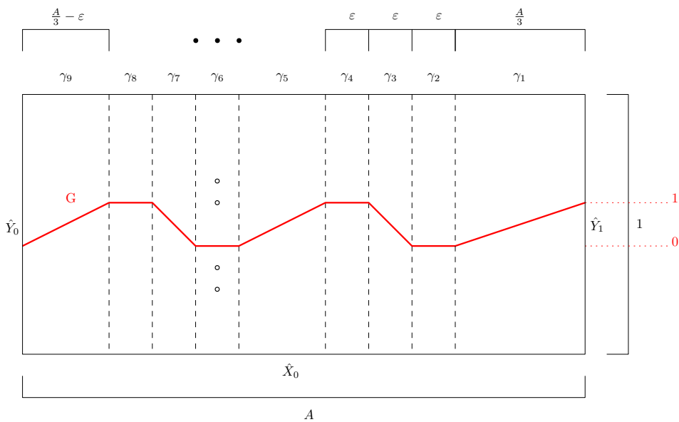
Figure 5. Partition and function in the case k = 3 .
