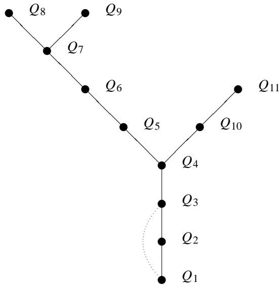
Figure 1. The proximity graph of K
