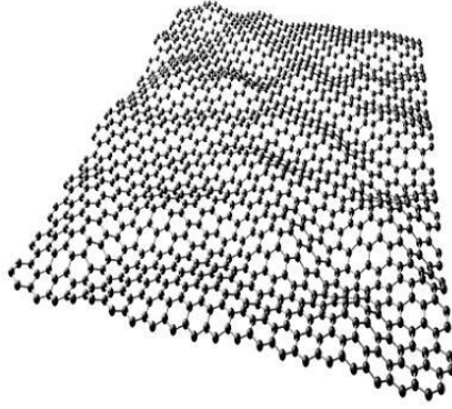
Figure 2. A deformed graphene mono-atomic layer resisting in-plane stretches (membrane effects) and curvature. Classical continuum models are no longer suitable, since there is no tangible thickness, cf. [75]. Graphene is thought to be the strongest among all known materials. Nevertheless, it is soft in the sense that it can be easily bent due to its one-atom-thin nature.
