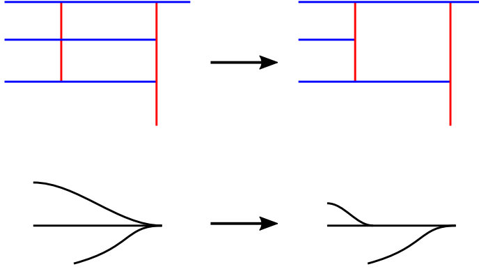
Figure 8. Performing elementary folding moves on \tau_j to obtain \tau_{j+1} .
