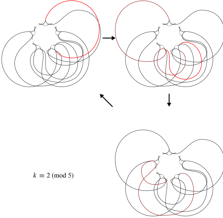
Figure 20. Folding sequence of train tracks in the second family of examples.
