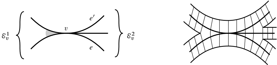
Figure 1. A train track and its tie neighborhood near a switch.
