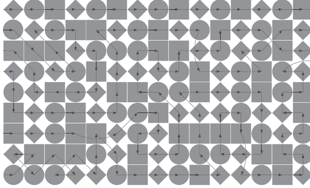
Figure 2. Representation of a finite pattern in a of configuration in Y[X_2(\mathbb{Z}, \mathbb{Z}^2)] . Here, A is the alphabet {circle, square, rhombus}, and Y \subset A^{\mathbb{Z}} is the subshift of all sequences that alternate circle, square, and rhombus in that order.
