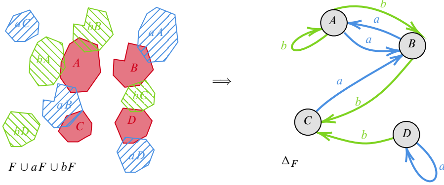
Figure 5. An example of the construction of an adjacency digraph. Here, \pi_0(F) = \{A, B, C, D\} and S_F = \{a, b, a^{-1}, b^{-1}\} . Due to symmetry we have not drawn the translates of F by a^{-1} or b^{-1} , nor the corresponding edges of \Delta_F .
