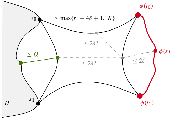
Figure 4. The point \phi(s) cannot be too far from H .
