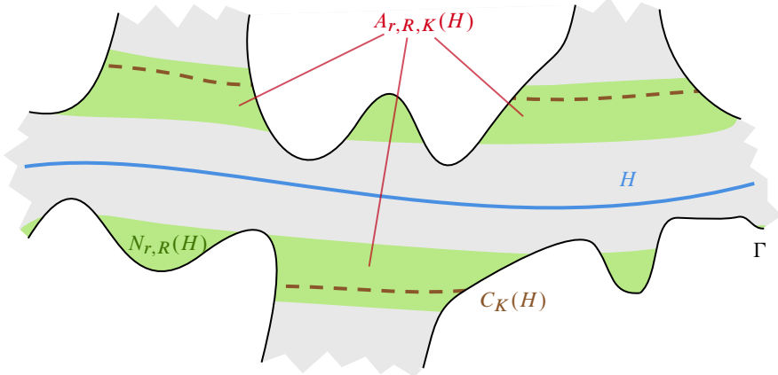
Figure 1. The region A_{r,R,K}(H) surrounding H . In this cartoon, H is depicted as a line for illustrative purposes.
