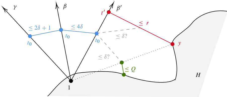
Figure 2. Bounding the distance between \gamma(t_0) and H .
