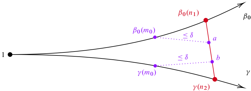
Figure 3. The point a is closer to \beta_0(n_1) than b .
