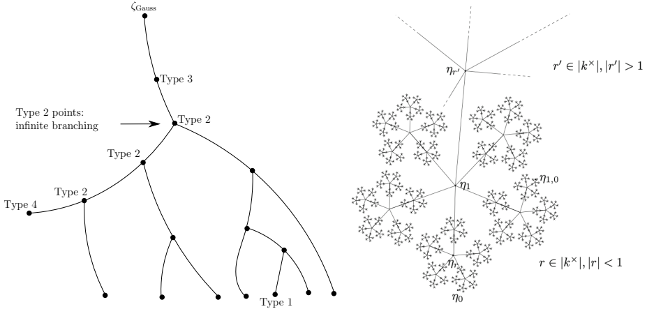
Figure 1. The Berkovich affine line. Picture on the right is taken from [26].
