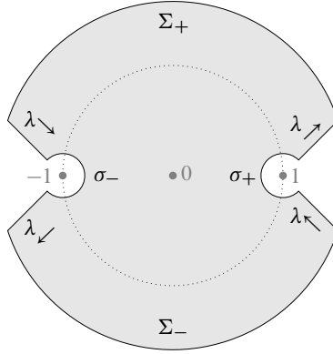
Fig. 1. The contour \gamma .
