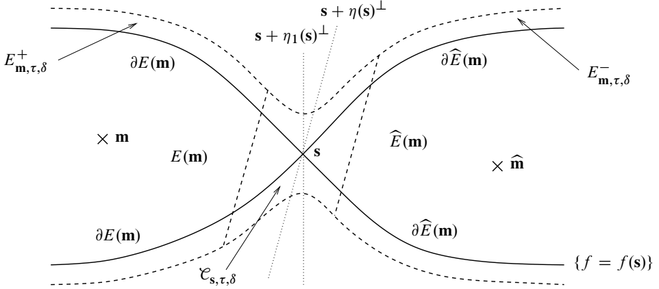
Fig. 4.2. Representation of the Morse function f near a point \mathbf{s} \in \mathbf{j}(\mathbf{m}) \cap \widehat{E}(\mathbf{m}) when the latter set is nonempty. Here, \eta_1(\mathbf{s}) denotes an eigenvector of \text{Hess } f(\mathbf{s}) associated with its negative eigenvalue.
