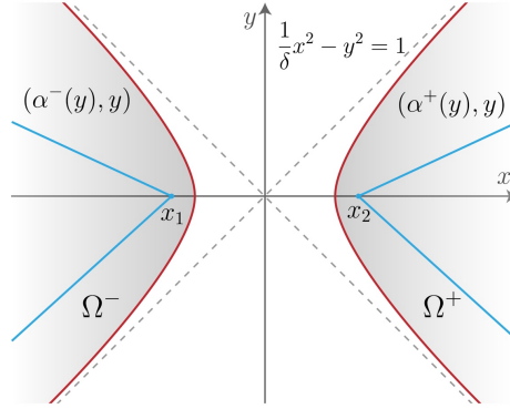
Fig. 2.1. The curves (\alpha^\pm(y), y) in \mathbb{R}^2 .
