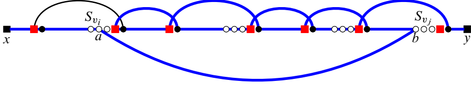
Fig. 2. The shorter path P' is drawn in blue, the special vertices are represented with red squares, while the vertices after them on P are represented with black dots. The vertices in the sets S_v are represented with white dots. Also note the following about the black dots and red squares which are between a and b in P . It could be that one of these black dots and the red square which is after it in our drawing are the same vertex. However, the construction of the path P' remains the same (for example, the fourth black dot and the fifth red square could be the same vertex). Notice also in the drawing that some of the red squares do not have a corresponding set of white dots. These are precisely those special vertices which are in U_c \cup \{v_1\} .
