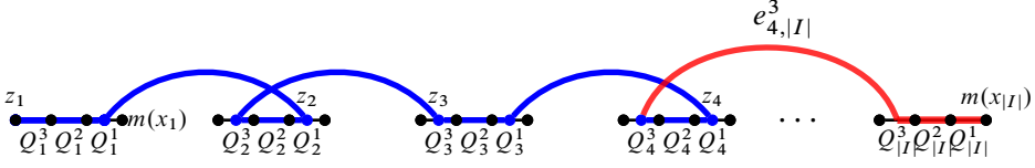
Fig. 3. The thick blue path represents the path R_4 , and adding to it the red path creates R'_4 .
