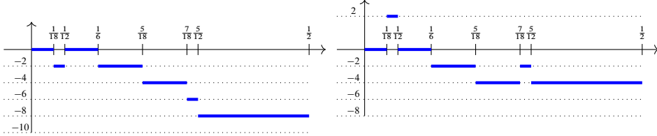
Fig. 3.4. The signature functions x \mapsto \sigma(e^{2\pi ix}) , x \in [0, 1/2] , for links of Figure 3.3.
