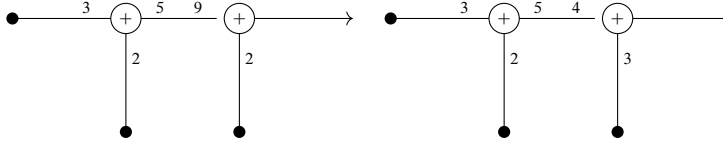
Fig. 3.3. The two links of [3] represented as graph links of [6].
