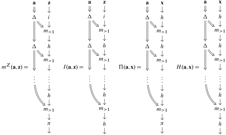
Fig. 2.1. The maps appearing in the homological perturbation lemma for A_\infty -modules. The notation is introduced in [25, Section 2]. Briefly, a single arrow represents an element of \mathcal{A}M , while a double arrow represents an element of \bigoplus_i \mathcal{A}^{\otimes i} .
