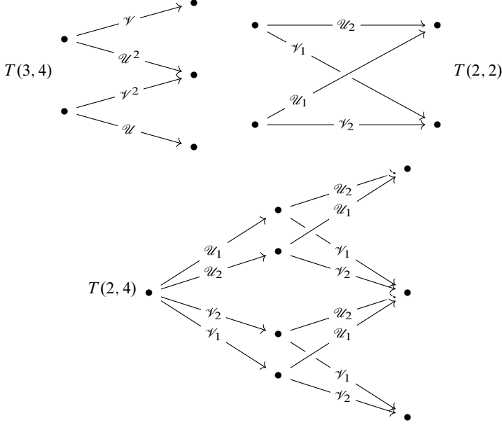
Fig. 1.1. The knot and link Floer complexes of T(3, 4) , T(2, 2) and T(2, 4) . Each dot denotes a generator in a free basis. The horizontal direction indicates the grading of the free resolution.
