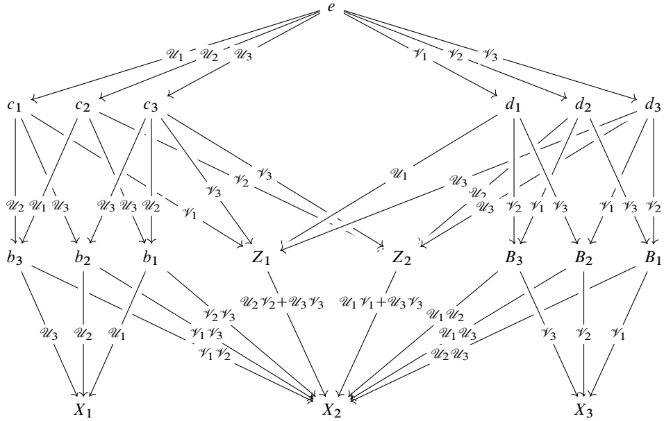
Fig. 7.1. The complex \mathcal{CFL}(T(3, 3)) as a free resolution.
