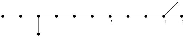
Fig. 3.2. Plumbing graph of the second knot in Proposition 3.20 (b). All weights that are not explicitly marked have value -2 .
