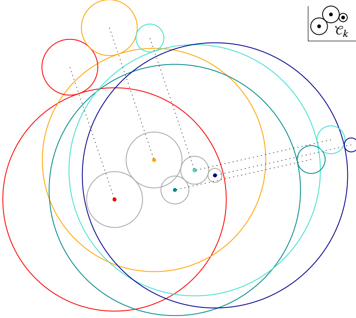
Fig. 5. Illustration for the construction of the family \mathcal{C}_{k+1} from \mathcal{C}_k . Gray circles represent a part of the set X \subset \mathbb{R}^3 containing two homothetic copies of T_0 in \mathcal{T} , both such that r_T^* = 0 (for clarity of the illustration). The family \mathcal{C}_{k+1} contains a (large) circle for each point in X and a homothetic copy of \mathcal{C}_k for each homothetic copy of T_0 in \mathcal{T} .
