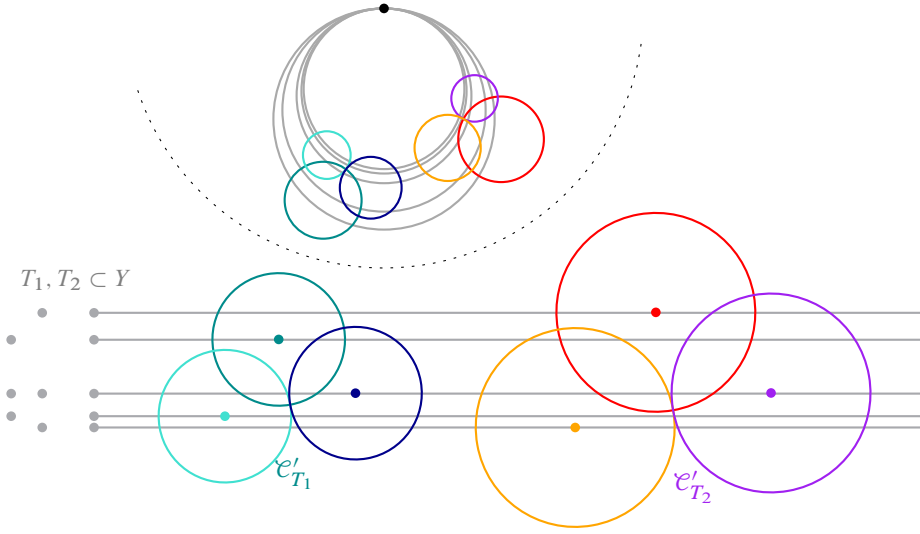
Fig. 4. Illustration for steps (3)–(5) in the proof of Theorem 8 for \theta = \frac{\pi}{2} : Construction of a preliminary family from Y and the result after inversion with respect to the dotted circle. Note that the set Y consists of two homothetic copies of the set T_0 from Figure 3 that have one element in common.
