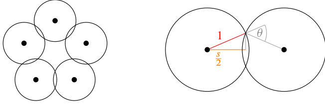
Fig. 2. In a regular n -gon of sidelength s , the circles intersect at an angle of \theta = \pi - 2 \arcsin(\frac{s}{2}) .
