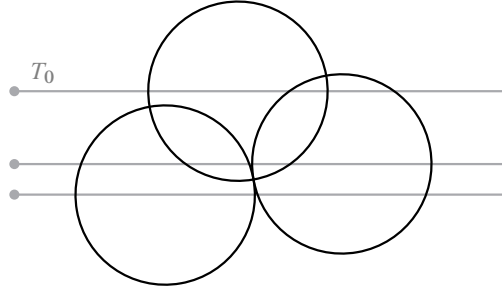
Fig. 3. Construction of the set T_0 for \theta = \frac{\pi}{2} .
