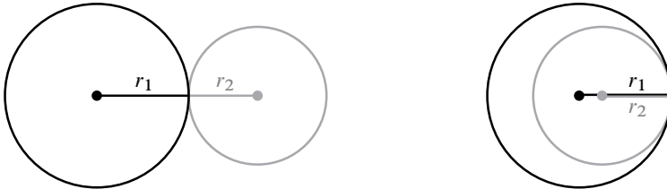
Fig. 6. External and internal tangency of circles.
