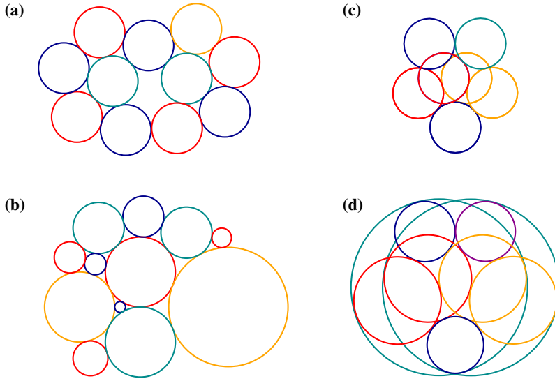
Fig. 1. An illustration of the four coloring problems of tangency graphs of constellations: (a) a penny graph, (b) a coin graph, (c) an overlapping penny graph, and (d) a general constellation as in the circle problem.
